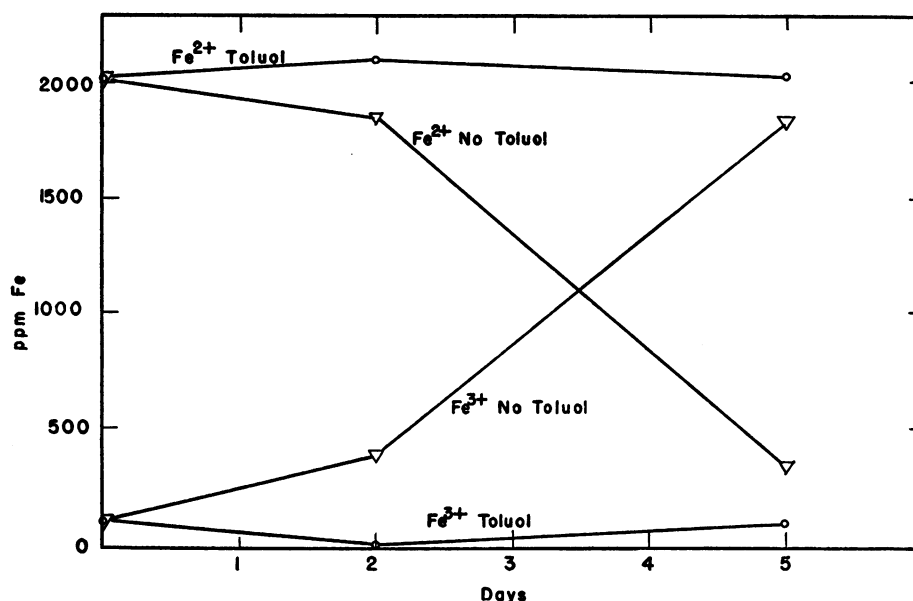
Figure 4. Iron transformations in artificial acid mine water, distilled water base, inoculated with a pure culture of iron-oxidizing bacterium.
