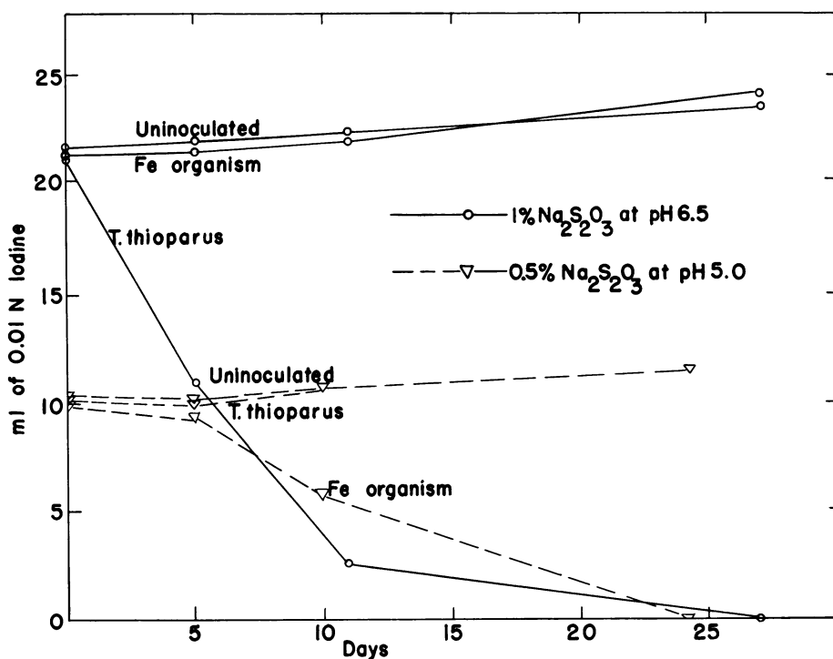
Figure 2. Sodium thiosulfate utilization (titration with 0.01 N I_2 ) and pH change by iron-oxidizing bacterium and T. thioparus in 0.5 per cent Na_2S_2O_3 medium at initial pH 5.0 and in 1 per cent Na_2S_2O_3 medium at initial pH 6.5.
